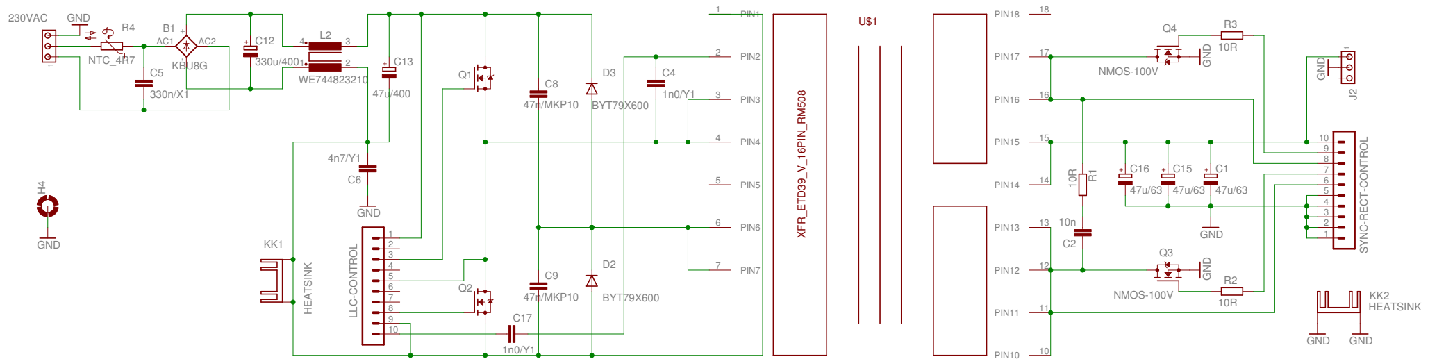
230V-LLC-converter, main board
