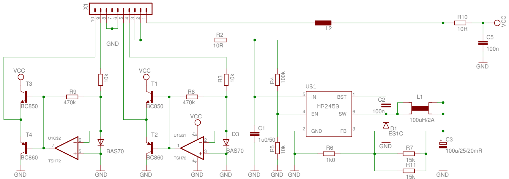
230V-LLC-Converter, sync rect control
