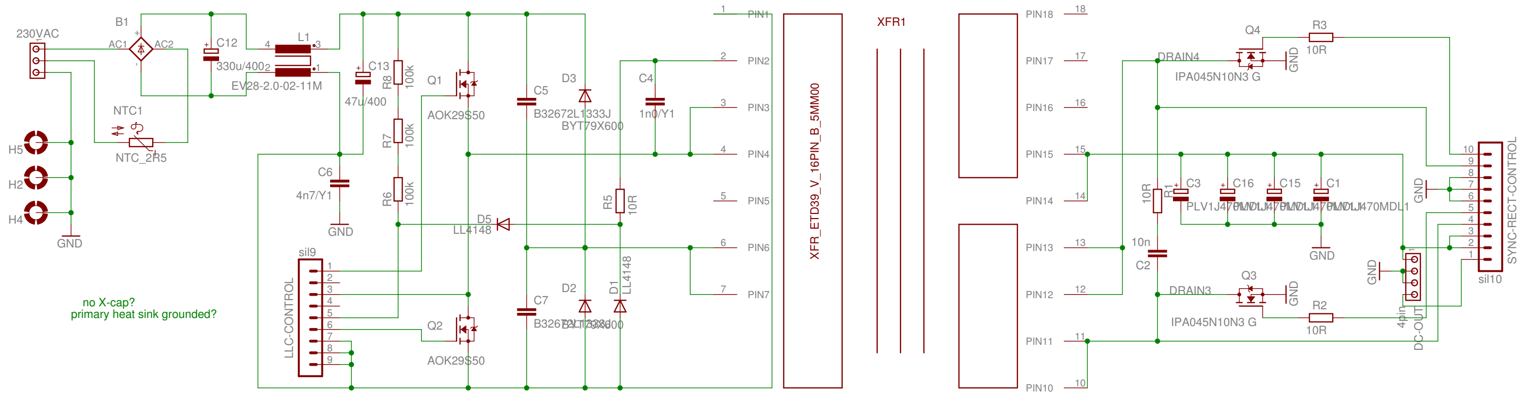
230V-LLC-converter, main board, 2016-08-17
